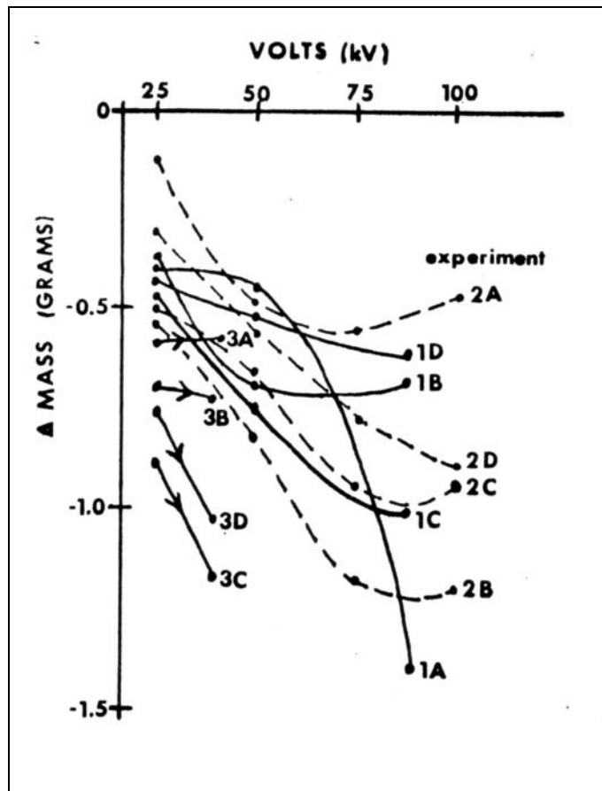
Figure 7: Graph of the unidirectional forces created by the change in voltage with a parallel plate capacitor relative to the earth. The graph indicates that the direction was constant, independent of polarity and orientation.
